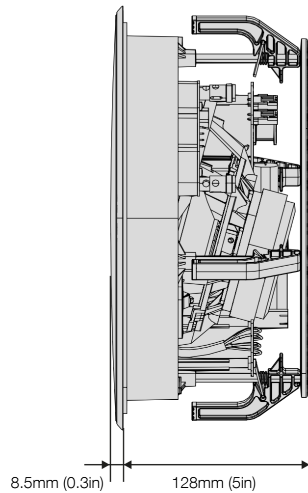
SIDE GRILLE ON
