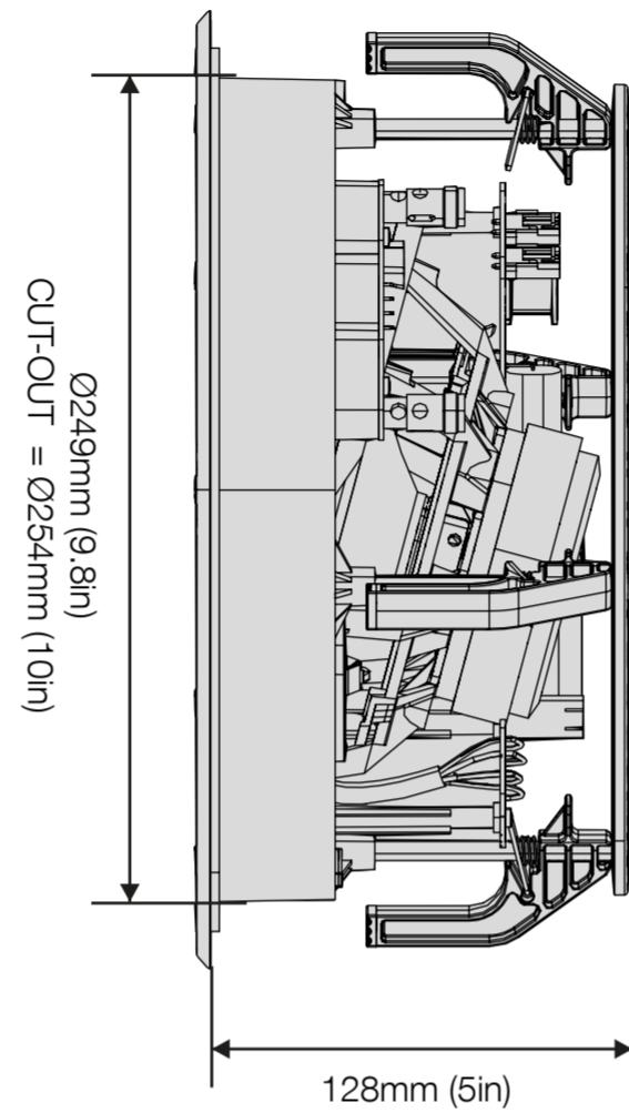
SIDE GRILLE OFF
